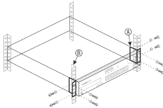
Figure 3: Rack-mount installation
