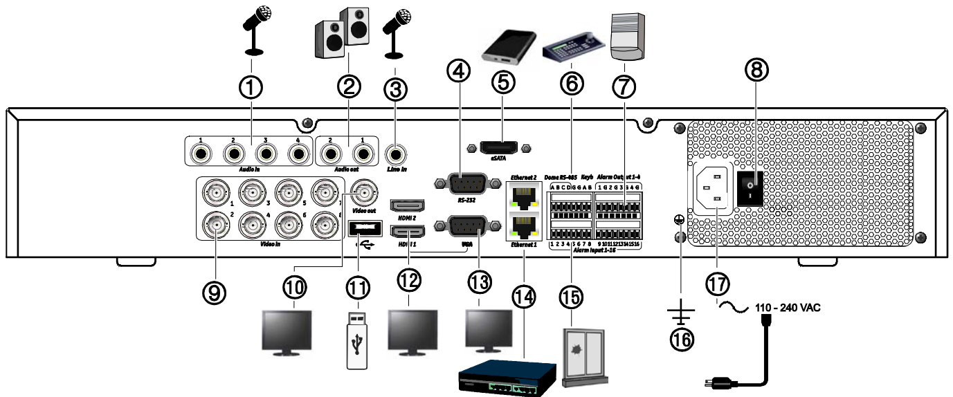
Figure 2: TVR 45HD back panel connections (8-channel models shown)
