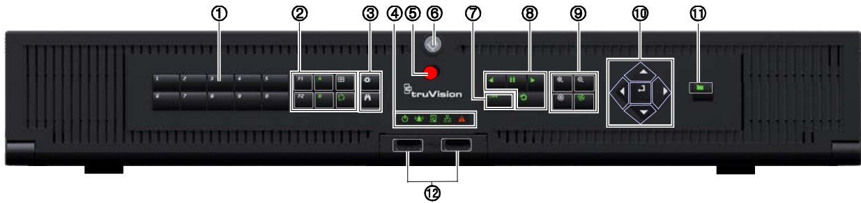
Figure 4: TVR 45HD front panel (8-channel model shown)
